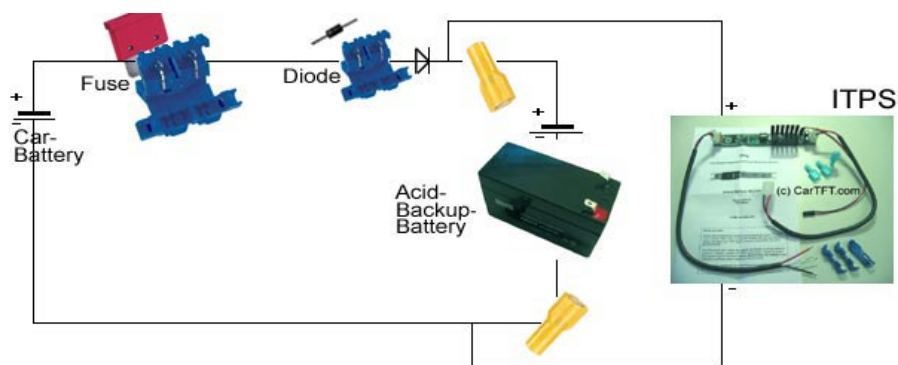
Backup-Battery-Wiring-Diagram
